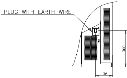
VIEW A(1/10)
